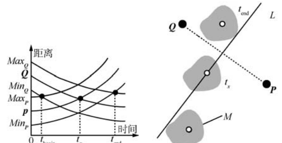
(a) 距离曲线相交实例 (b) 不确定区域变化示意图 (a) Example of intersection of the distance curve (b) Example of the change of uncertain area
