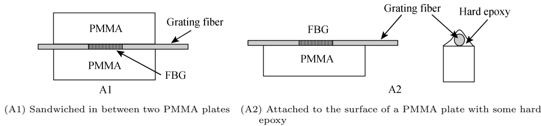
Fig. 2 FBG is fixed with hard epoxy resin
