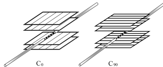
Fig. 4 FBG embedded into CFRC, with grating fiber running 0^{\circ} ( C_0 ) and 90^{\circ} ( C_{90} ) to the carbon fiber
