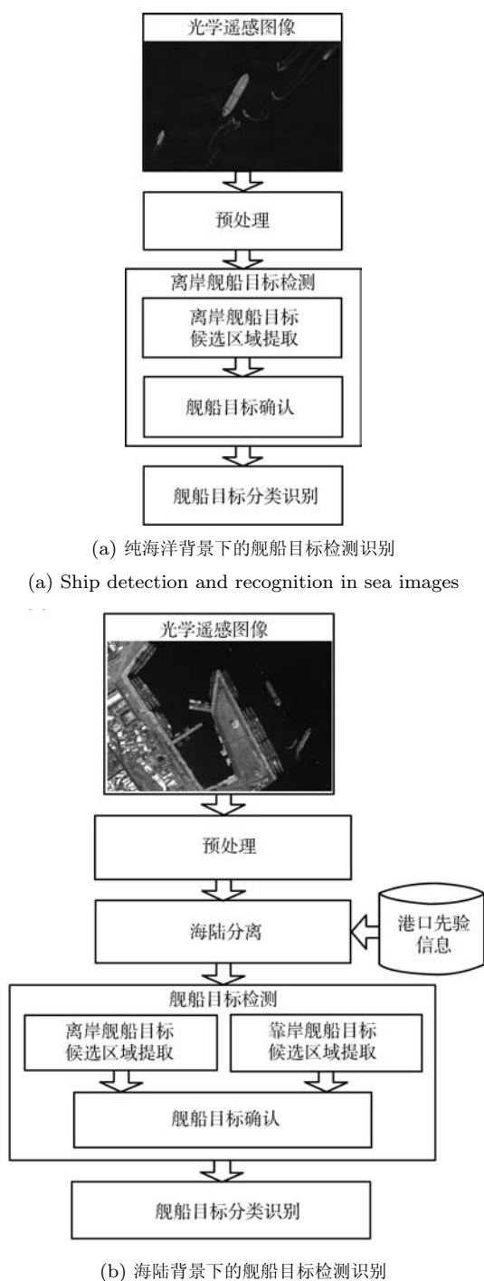
图 1 光学遥感图像舰船目标检测识别的一般处理框架 Fig. 1 General framework for ship detection and recognition in optical remotely sensed images
