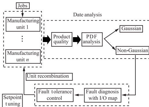
Fig. 14 A data-driven system approach for fault diagnosis and fault tolerance control
