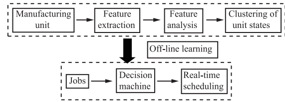
Fig. 15 A data-driven system approach for dynamic or real-time scheduling in presence of uncertain events or disturbances
