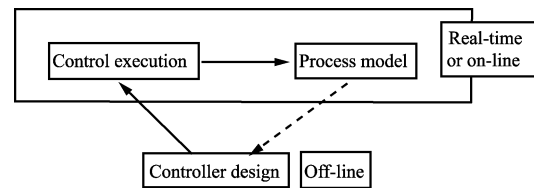
Fig. 11 A traditional controller design method in which the design model is the same as the physical process model
