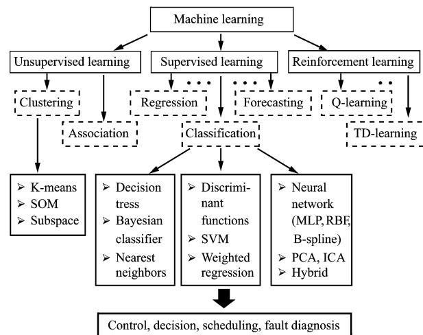
Fig. 3 The outline of machine learning approaches that could be relevant to data-driven systems in control, decision making, scheduling, and fault diagnosis
