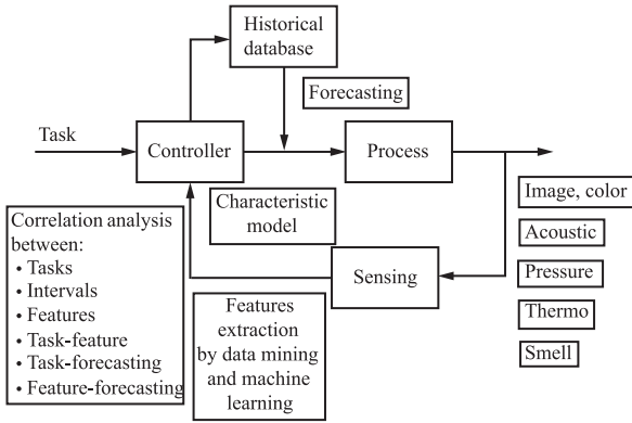
Fig. 13 A prototype of data-driven control systems that can sense and handle heterogeneous data, conduct feature analysis and extraction, perform correlation analysis, characteristic pattern matching, and forecasting
