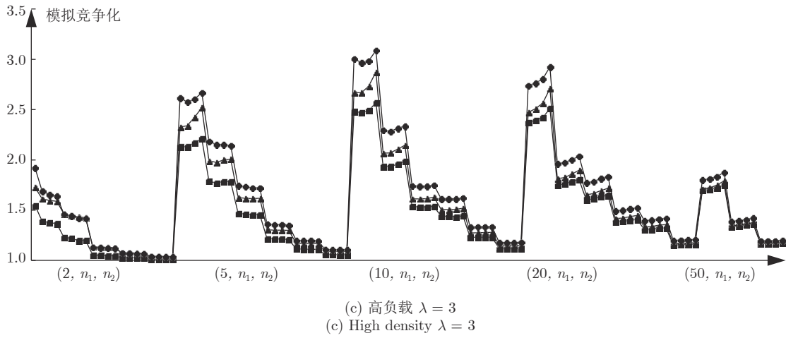
图 7 \alpha AD-I 算法在一般实例下的实验结果 Fig. 7 The experimental results of \alpha AD-I in general instances
