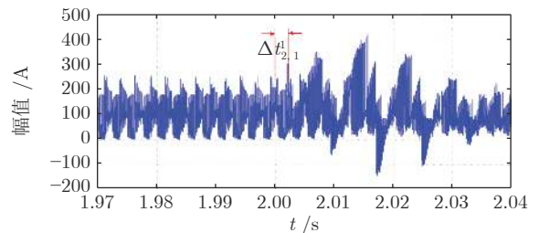
(b) 观测点 2 电流时域波形 (b) The time domain waveform of the current at observation point 2
