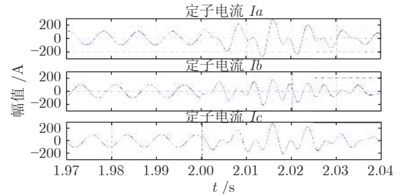
(a) 观测点 1 电流时域波形 (a) The time domain waveform of the current at observation point 1
