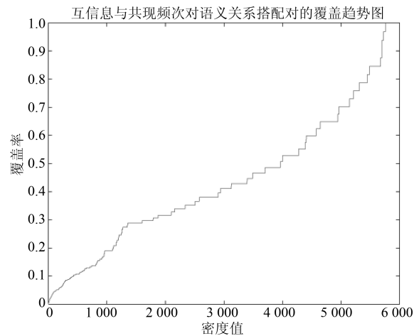
图 6 互信息与共现频次对语义关系搭配对的覆盖趋势图 Fig. 6 The coverage trend figure of mutual information and co-occurrence frequency for semantic collocation
