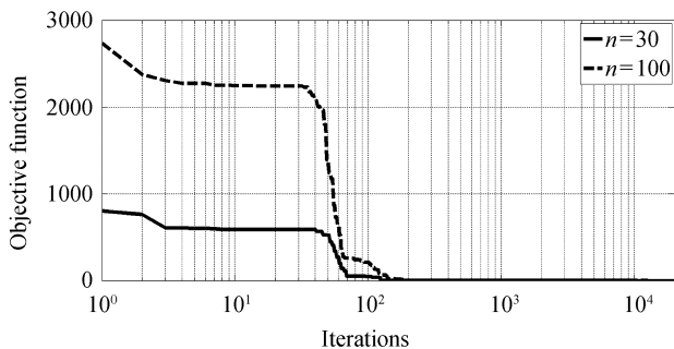
Fig. 5. Iteration curve of griewank.
