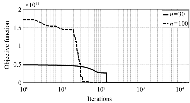
Fig. 6. Iteration curve of rosenbrock.
