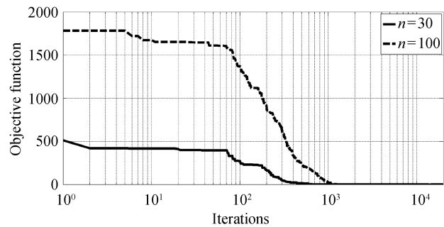
Fig. 7. Iteration curve of restrigin.
