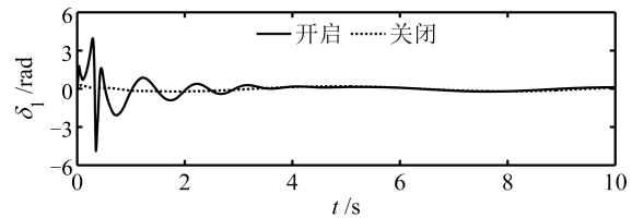
(a) Elastic deformation of the base
