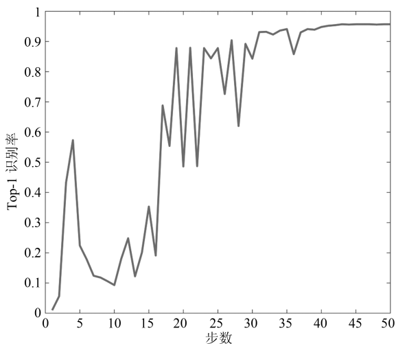
(a) Top-1 识别率
